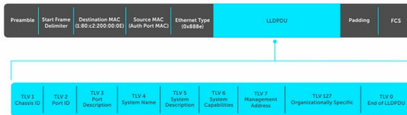
Figure 67. LLDPDU Frame
